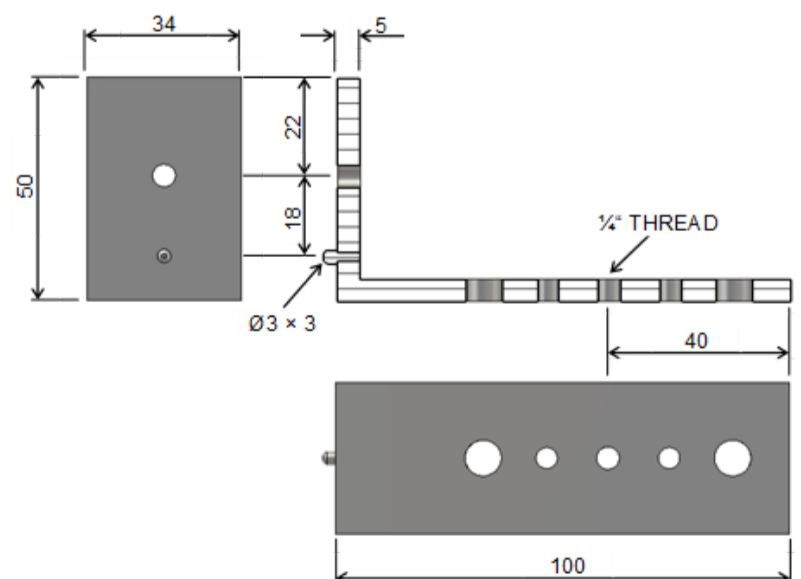
Mounting flange
