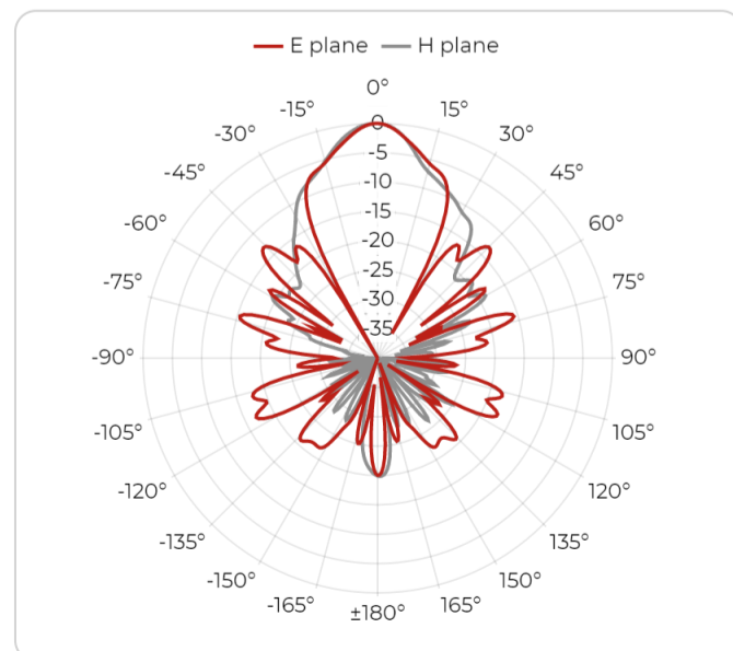
5.5 GHz
