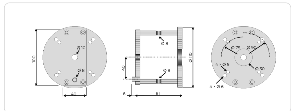
Mounting flange
